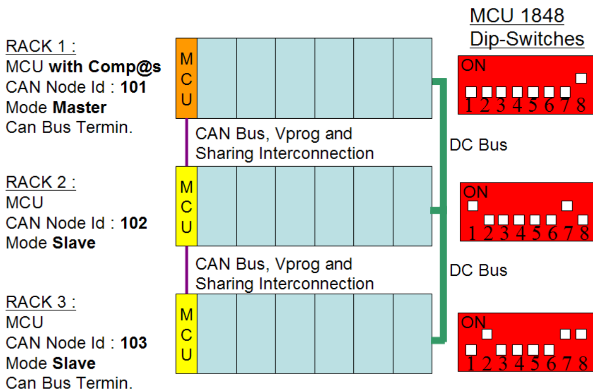
Figure 68 Example with a system of 3 shelves of 6x1800W rectifiers
