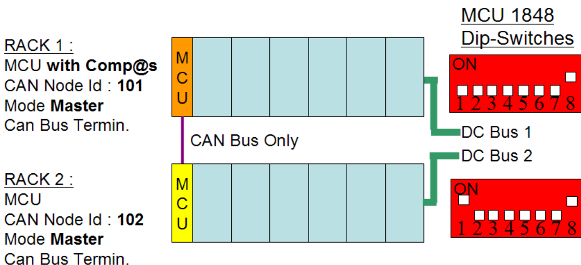
Figure 69 Example with a system with 2 shelves of 6x1800W rectifiers
