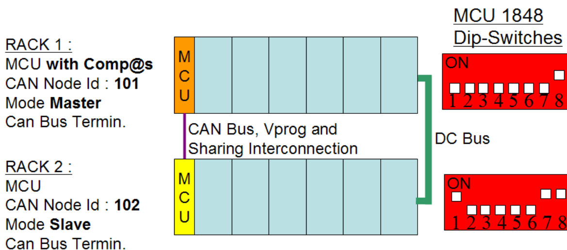
Figure 67 Example with a system with 2 shelves of 6x1800W rectifiers
